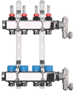
R553FS Debi Göstergeli Paslanmaz Kollektör Stainless Steel Manifold With Dynamic Flow Balancing
